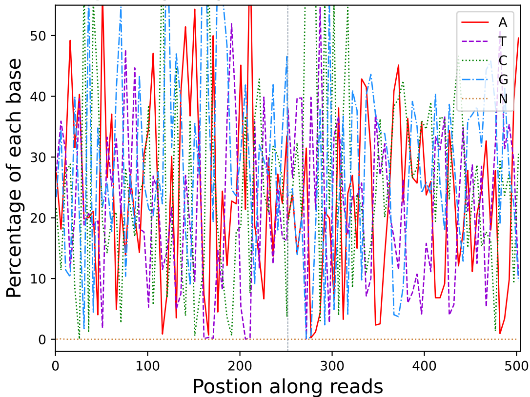
Base percentage along reads (CK2)
